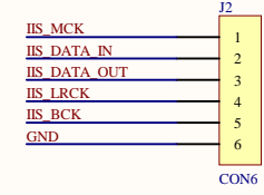
I2S Digital audio output
